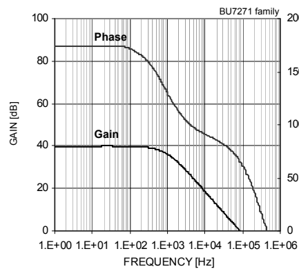
Fig.46 Gain – Frequency
