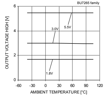
Fig.6 Output Voltage High - Ambient Temperature (RL=10[kΩ])
