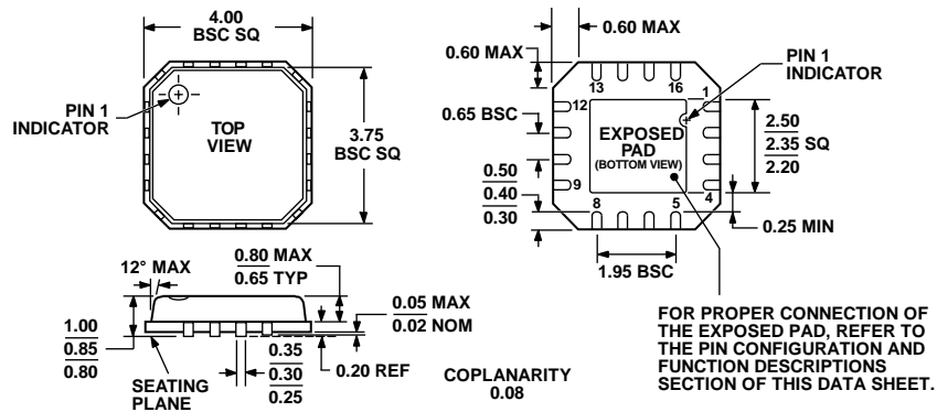
Figure 49. 16-Lead Lead Frame Chip Scale Package [LFCSP_VQ] 4 mm x 4 mm Body, Very Thin Quad (CP-16-10) Dimensions shown in millimeters
