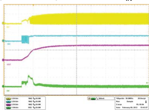
Figure 21. Startup after enable @ V_{IN}=1.8\text{ V}
