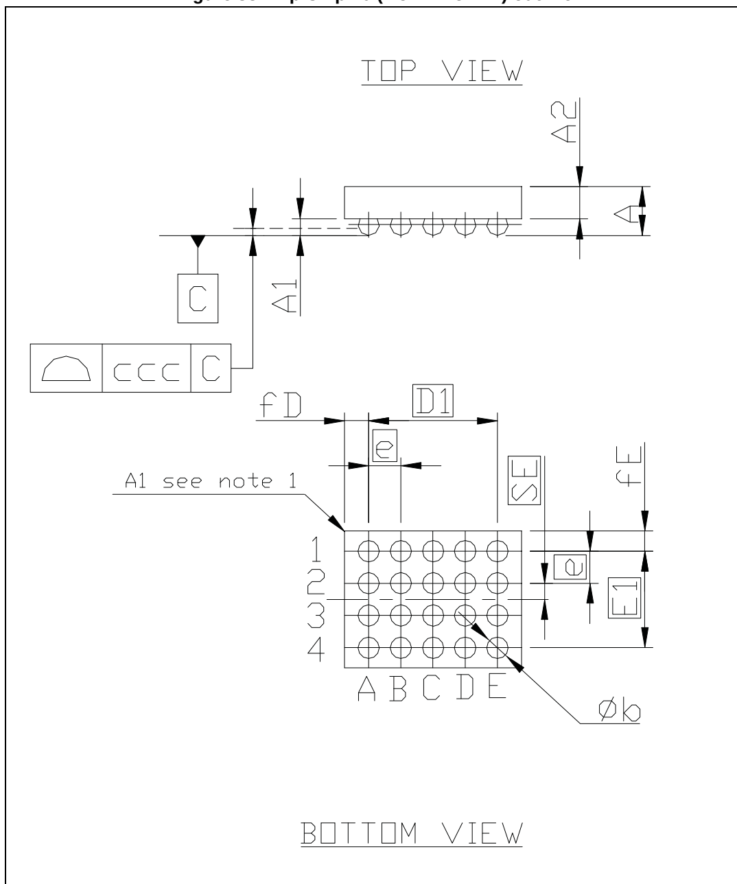
Figure 38. Flip Chip 20 (2.5 x 1.75 mm) outline
