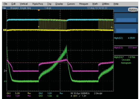
Figure 25. OCP threshold
