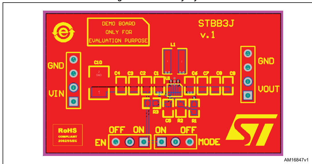
Figure 33. Top layer
