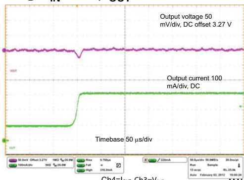
Figure 19. Load transient response @ V_{IN}=5.5\text{ V} , I_{OUT} = 100\text{ to }300\text{ mA}
