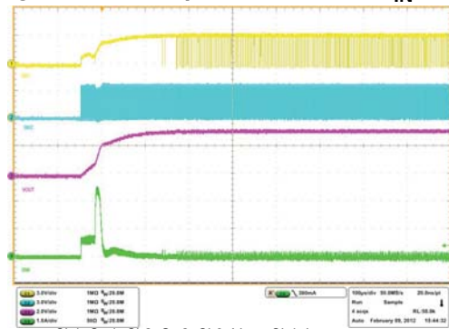
Figure 22. Startup after enable @ V_{IN}=3.6\text{ V}
