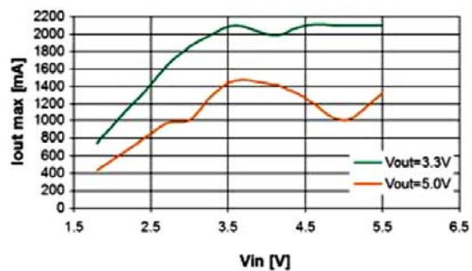
Figure 10. Maximum output current vs. input voltage
