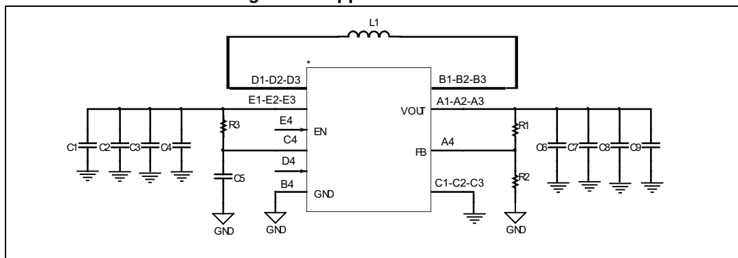
Figure 30. Application schematic
