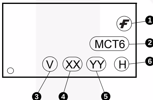
Figure 10. Top Mark
