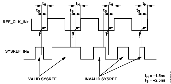
Figure 3. SYSREF\_IN\pm Setup and Hold Timing Examples, Relative to Device Clock
