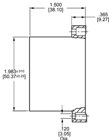
Receptacle Housing
