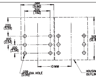
RECOMMENDED PC BOARD LAYOUT (Component Side) (.300 x .100) (7.62 mm) x (2.54)
