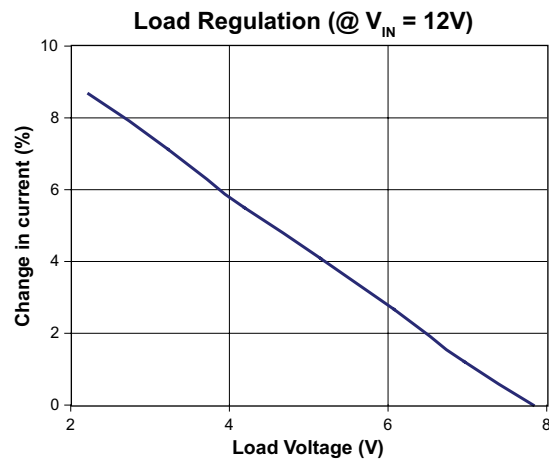
Fig. 8. Load Regulation of LED Current Plot
