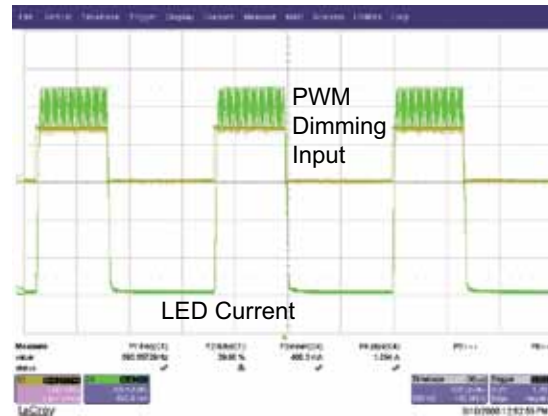
(a) PWM Dimming Performance
