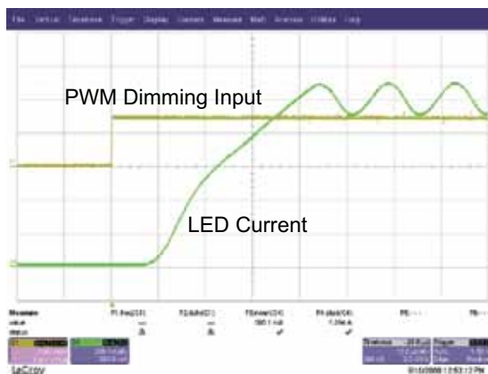
(b) PWM Dimming Rise Time
