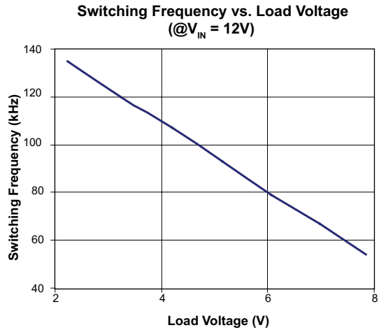
Fig. 9. Switching Frequency vs. Load Voltage Plot
