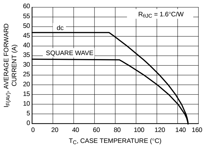
Figure 6. Current Derating
