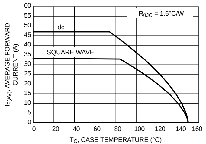
Figure 6. Current Derating
