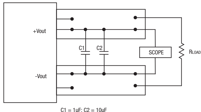
Figure 4. Measuring Output Ripple and Noise (PARD)
