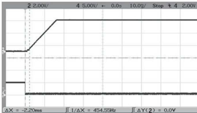
On/Off Enable Start-up (Vin = 48V, Vout = nom, Iout = 40A, Cload = 10000μf, Ta = +25°C) ch2 = Vout, ch4 = Enable
