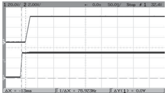
Start-up Delay (Vin = 48V, Vout = nom, Iout = 40A, Cload = 10000μf, Ta = +25°C) ch1 = Vin, ch2 = Vout
