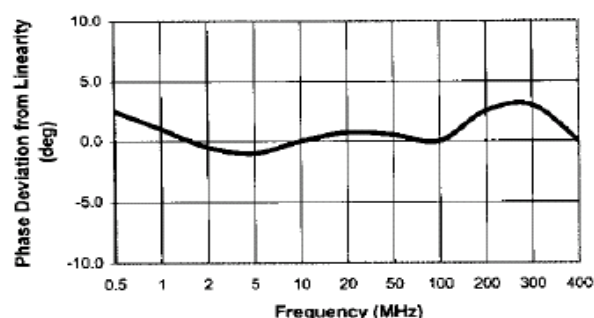
Phase Linearity
