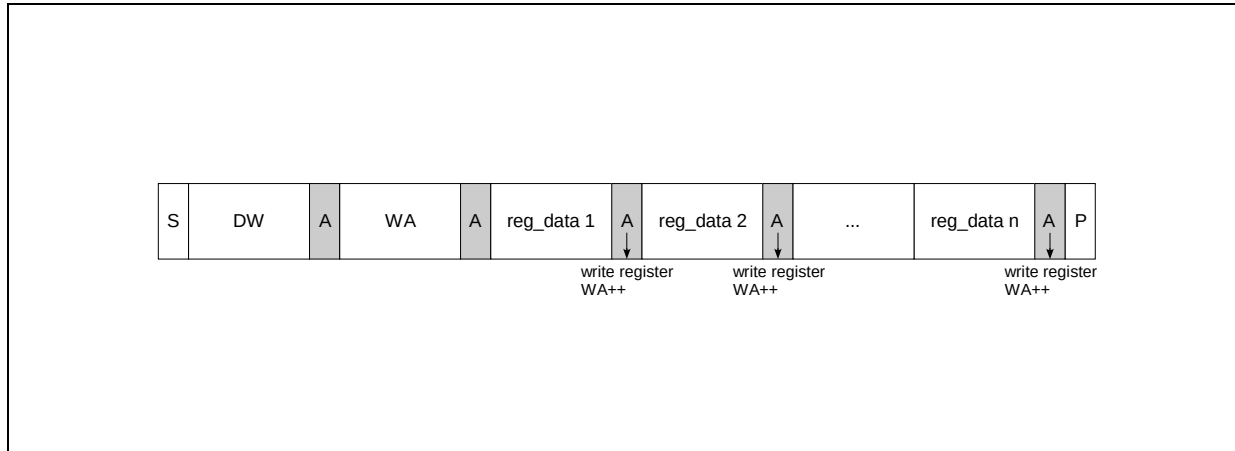
Figure 15. Page Write
