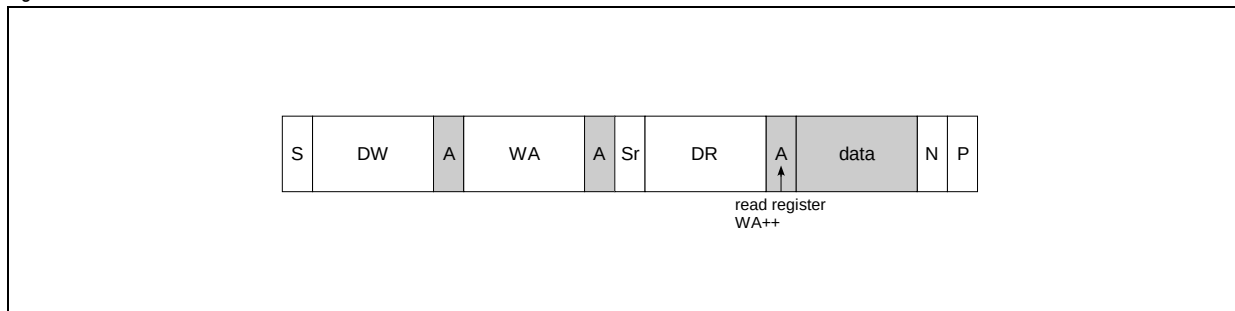
Figure 16. Random Read
