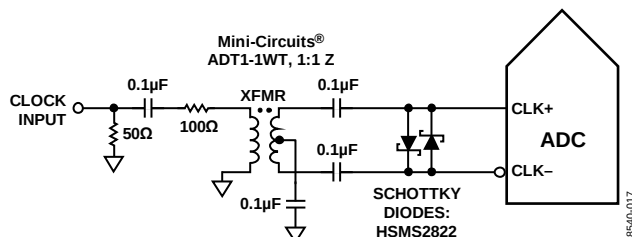
Figure 46. Transformer-Coupled Differential Clock (3 MHz to 200 MHz)
