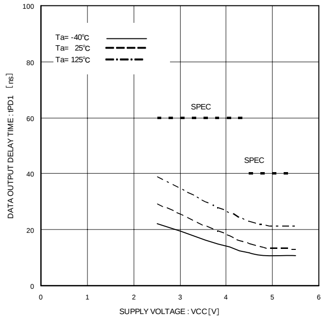
Figure 25. Data Output Delay Time t_{PD1} ( CL=100\text{pF} )
