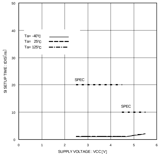
Figure 23. SI Setup Time t_{DIS}
