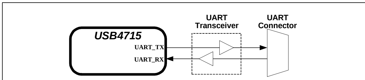
FIGURE 4-5: UART CONNECTIONS
