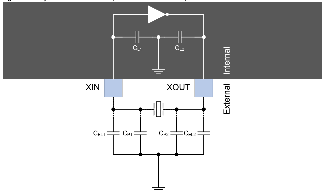
Figure 44-8. Crystal Circuit With Internal, External and Parasitic Capacitance
