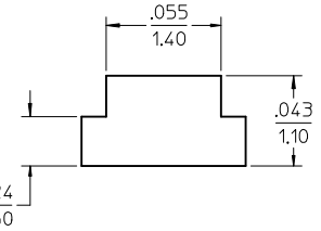
RECOMMENDED SMT 0805 LED DIMENSIONS SCALE 20:1 (SEE NOTE 1)
