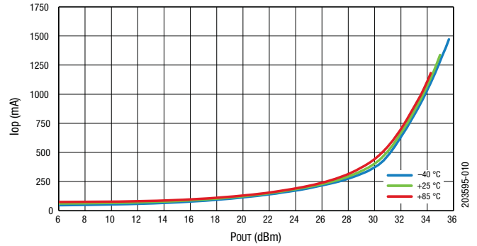
Figure 10. Operating Current vs POUT Across Temperature
