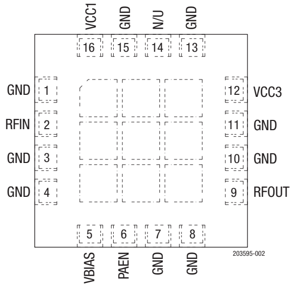
Figure 2. SKY66295-11 Pinout (Top View)
