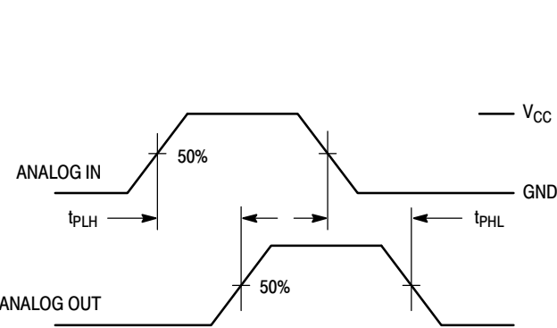
Figure 10. Propagation Delay, Analog In to Analog Out
