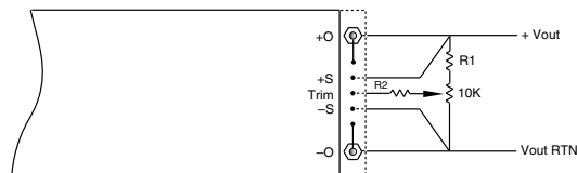
Resistor Values for Trimming Standard Output Voltages
