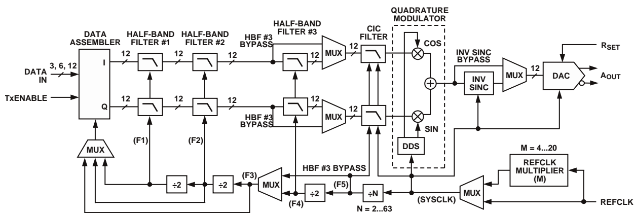
Figure 23. AD9856 Block Diagram
