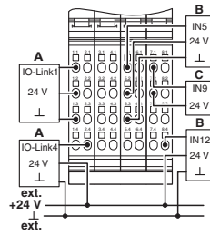
Connection diagram
