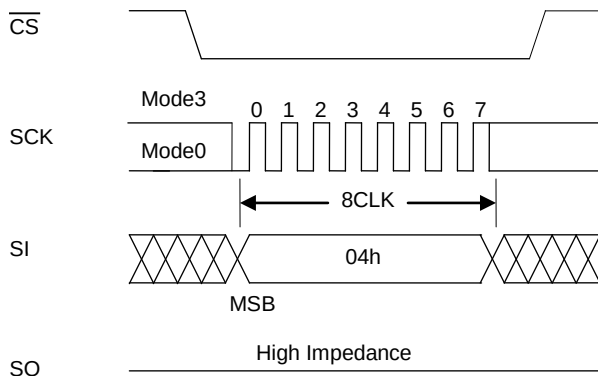
Figure 5. Write Disable (WRDI)
