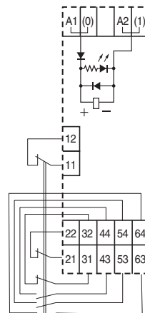
G7SA-3A3B Mounted
