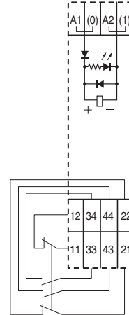
G7SA-2A2B Mounted
