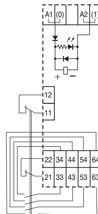
G7SA-4A2B Mounted
