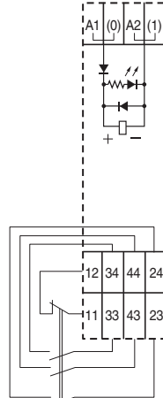
G7SA-3A1B Mounted
