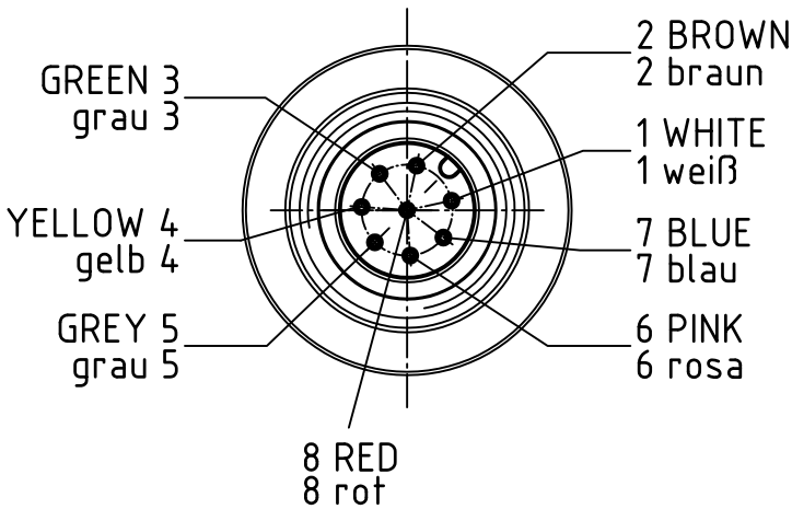
VIEW/Ansicht X MALE CABLE CONNECTOR/Kabelstecker 8-Pol
