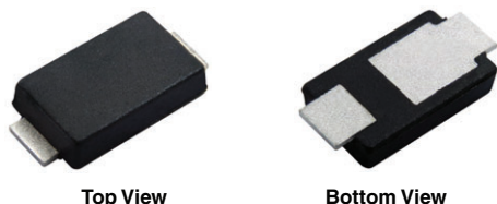
DO-221BC (SMPA)
