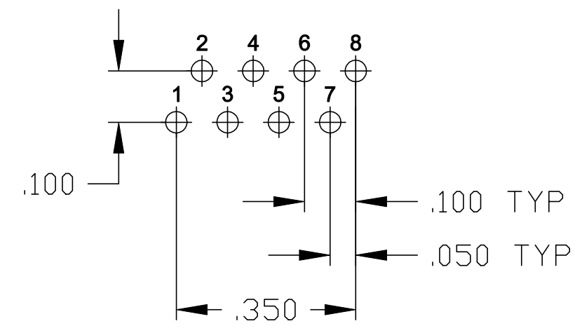
PIN DESIGNATIONS
