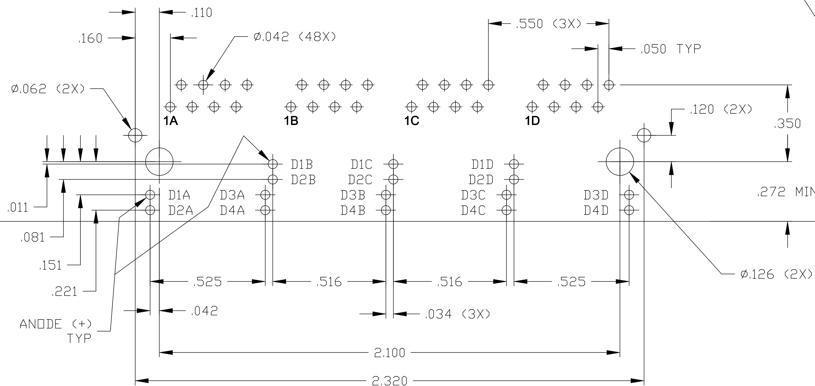
SUGGESTED PCB LAYOUT (COMPONENT SIDE)
