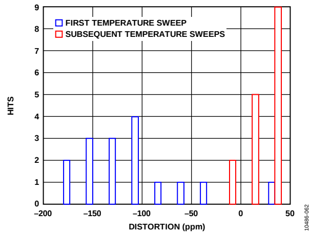
Figure 56. Thermal Hysteresis
