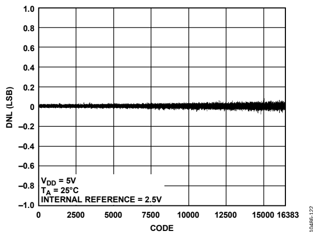
Figure 16. AD5695R DNL
