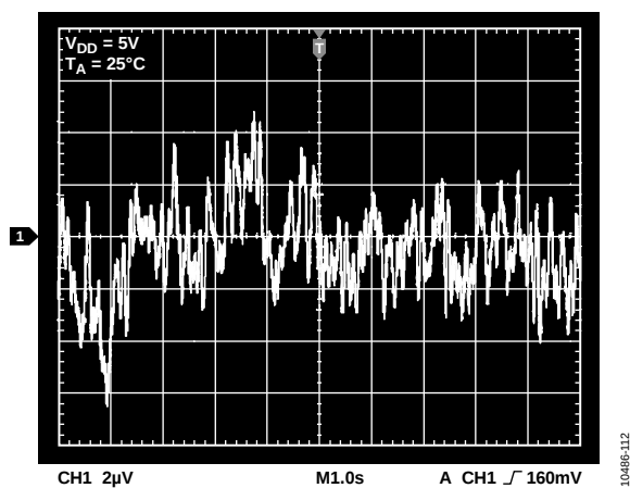
Figure 9. Internal Reference Noise, 0.1 Hz to 10 Hz
