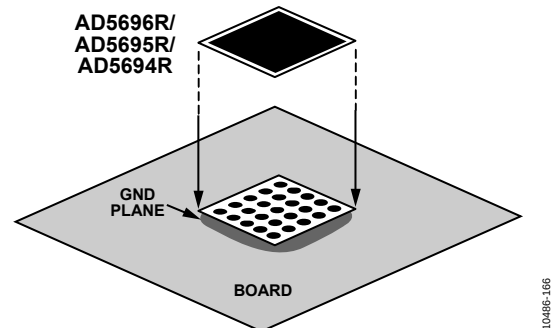
Figure 58. Paddle Connection to Board
