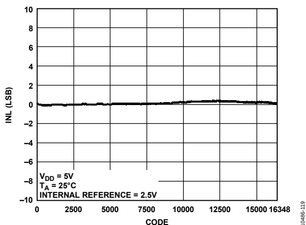
Figure 13. AD5695R INL
