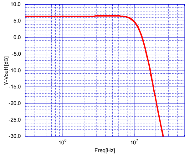
Voltage Gain vs. Frequency ( C_{in} \rightarrow V_{out} , V_{cc}=3V , T_a=25^\circ C )
