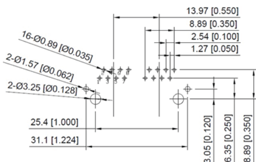
Top View Customer Board (COMP Side)
