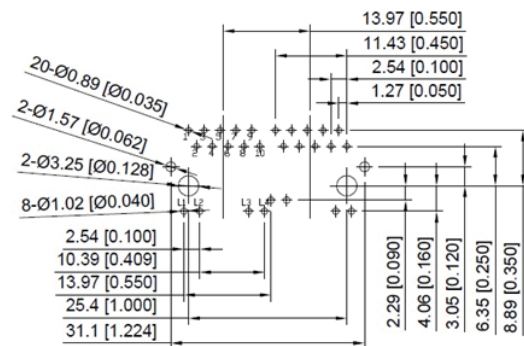
Top View Customer Board (COMP Side)
