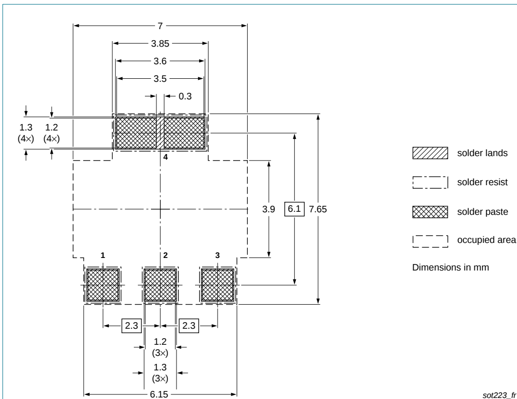
Fig 22. Reflow soldering footprint SOT223 (SC-73)
