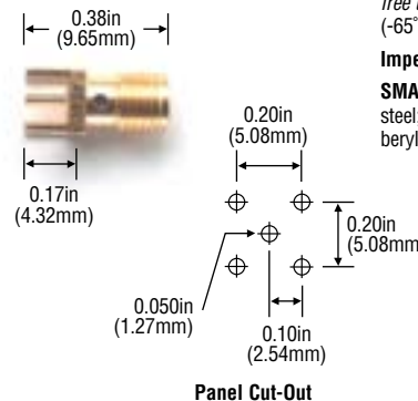
Panel Cut-Out
