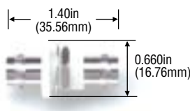
3846 See Cut-Out
