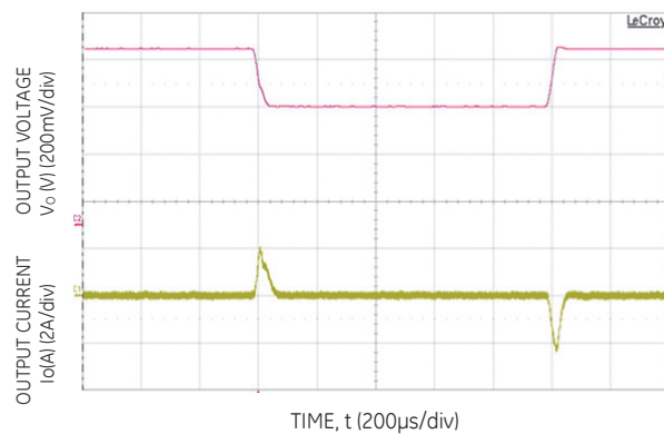
Figure 3. Transient Response to 0.1A/μs Dynamic Load Change from 50% to 75% to 50% of full load, Vin=48V
