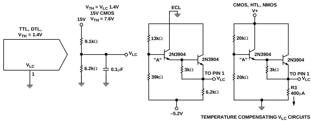
Figure 32. Interfacing with Various Logic Families
