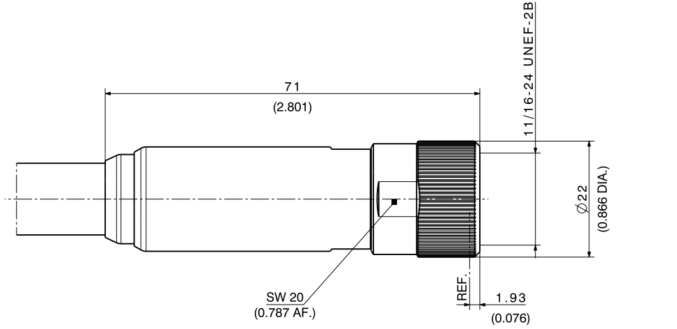
35 VF (3.5 mm ruggedized PORT female)
