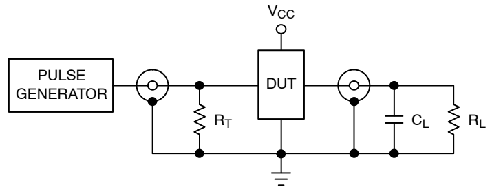
Figure 4. Test Circuit
