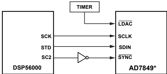
Figure 24. AD7849-to-DSP56000 Interface
