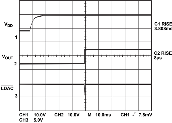
Figure 12. Turn-On Characteristics
