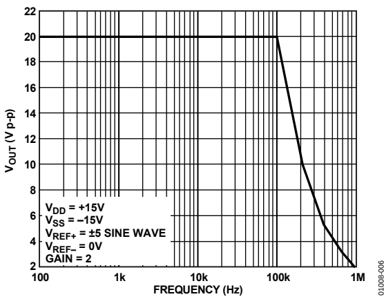
Figure 5. Large Signal Frequency Response
