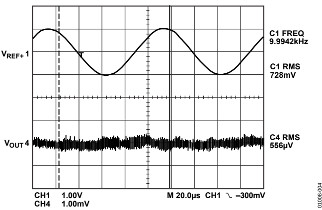
Figure 3. AC Feedthrough
