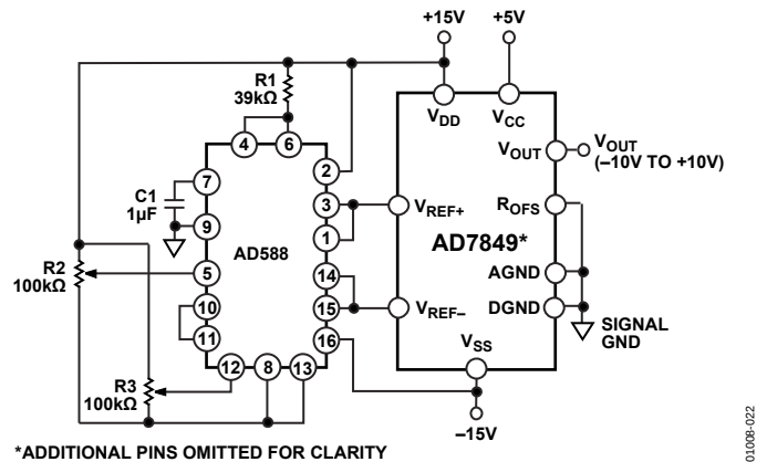
Figure 21. Bipolar \pm 10 \text{ V} Operation
