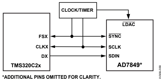
Figure 25. AD7849-to-TMS320C2x Interface
