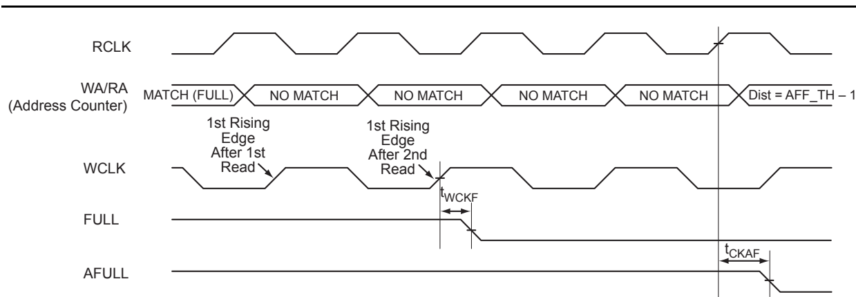
Figure 2-36 • FIFO FULL Flag and AFULL Flag Deassertion
