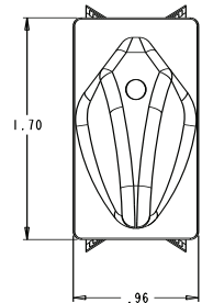
TERMINAL LOCATION AS VIEWED FROM THE BOTTOM OF THE SWITCH
