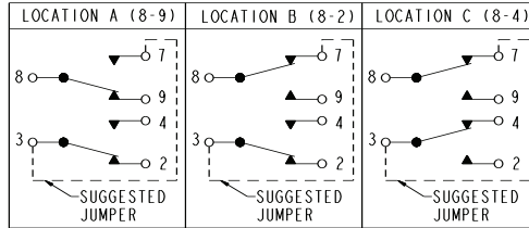
SPT SCHEMATIC USE R2XXXX7XXXX FOR (8-9), (8-2), (8-4) USE R2XXXX7XXXX FOR (OFF), (8-2), (8-4) USE R2XXXX7XXXX FOR (8-9), (8-2), (OFF)
