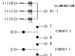
GENERIC SWITCH SCHEMATIC USE TERMINALS AS APPLICABLE TO PART NUMBER
