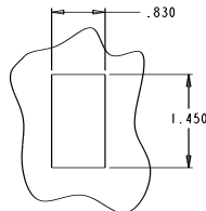
PANEL OPENING DETAIL SCALE 1:1 PANEL THICKNESS: .025 MIN. TO .187 MAX.
