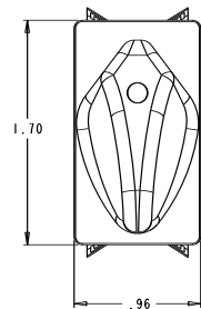
TERMINAL LOCATION AS VIEWED FROM THE BOTTOM OF THE SWITCH
