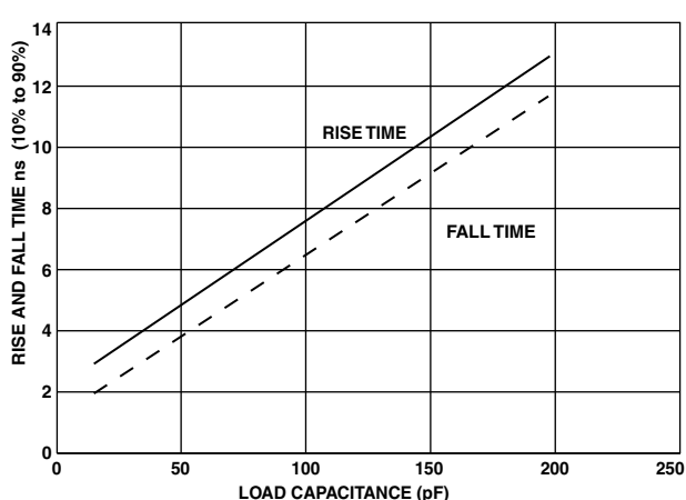
Figure 47. Typical Rise and Fall Times (10% to 90%) versus Load Capacitance for Driver D at V_{DDEXT} (max)
