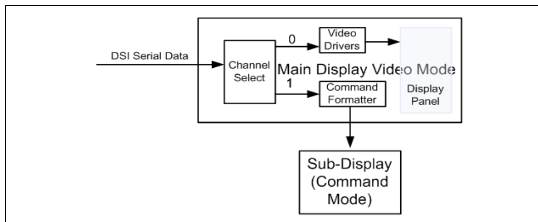
Figure 12. Sub-Display Connection
