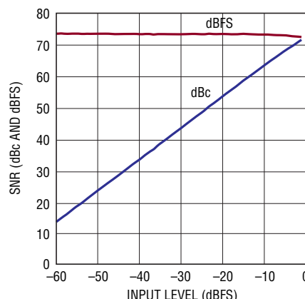
LTC2175-14: SNR vs Input Level, f_{IN} = 70\text{MHz} , 2V Range, 125Msps
