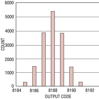
LTC2173-14: Shorted Input Histogram
