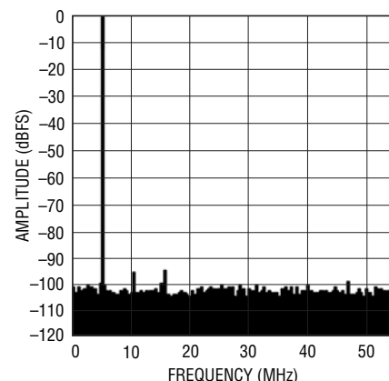
LTC2174-14: 8k Point FFT, f_{IN} = 5\text{MHz} , -1dBFS, 105Msps
