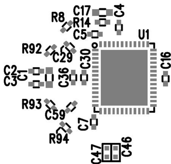
Silkscreen Top
