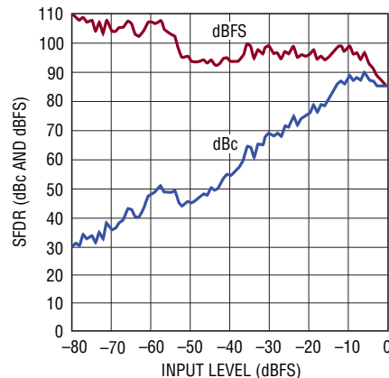
LTC2174-14: SFDR vs Input Level, f_{IN} = 70\text{MHz} , 2V Range, 105Mpsps
