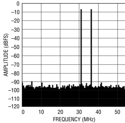
LTC2174-14: 8k Point 2-Tone FFT, f_{IN} = 70\text{MHz} , 75MHz, -1dBFS, 105Mpsps
