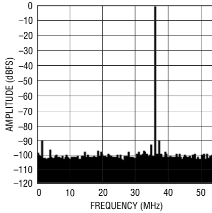
LTC2174-14: 8k Point FFT, f_{IN} = 70\text{MHz} -1dBFS, 105Mpsps
