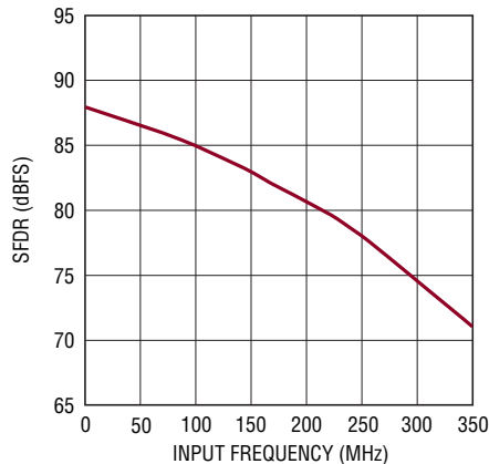
LTC2174-14: SFDR vs Input Frequency, -1dB, 2V Range, 105Mpsps
