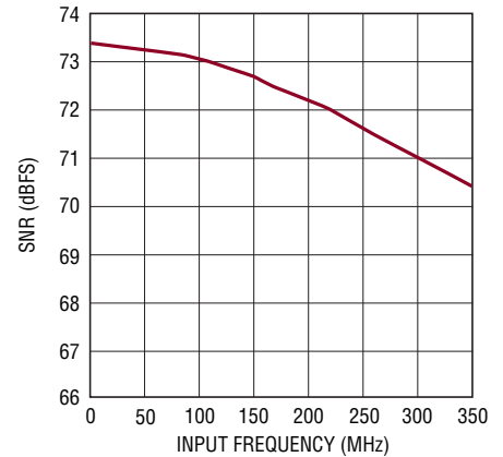
LTC2174-14: SNR vs Input Frequency, -1dB, 2V Range, 105Mpsps
